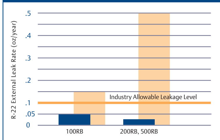
Emerson Refrigerant Solenoid Valve External Leak Test Results After Thermal Cycling
